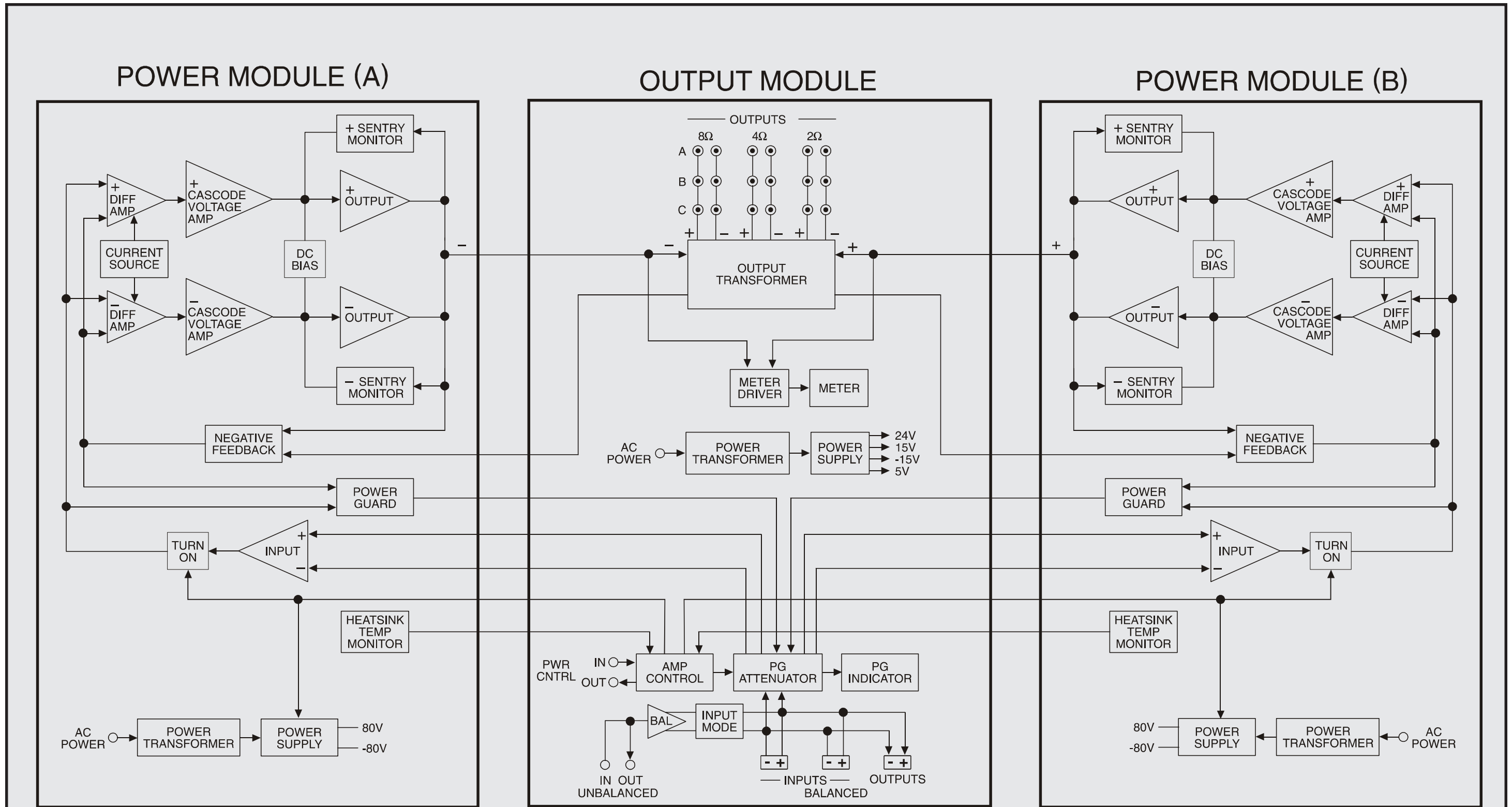
MC2KW Power Amplifier - Output Module with Power Modules A and B
