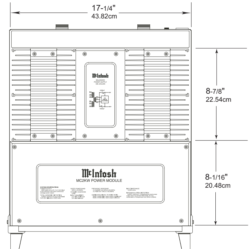
Top View of the MC2KW Power Module
