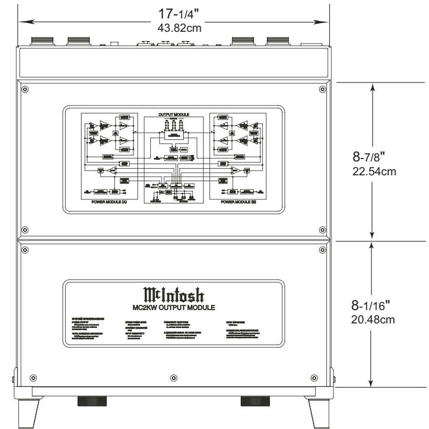
Top View of the MC2KW Output Module
