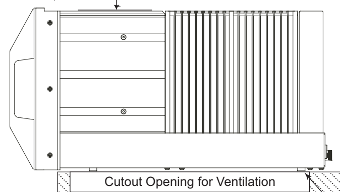
MC2KW Power Module Side View in Custom Cabinet
